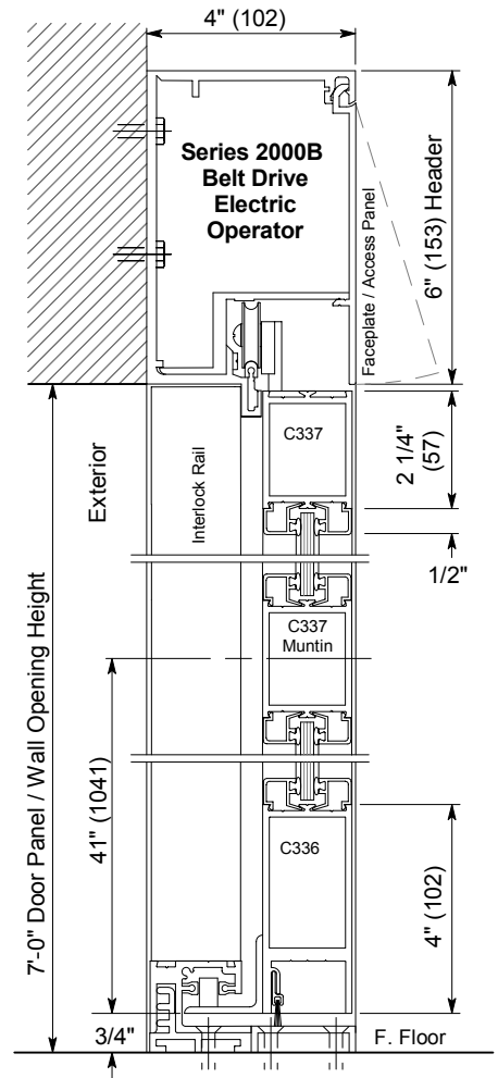
Vertical Section
