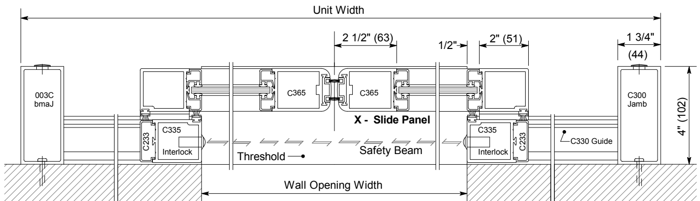
Horizontal Section
