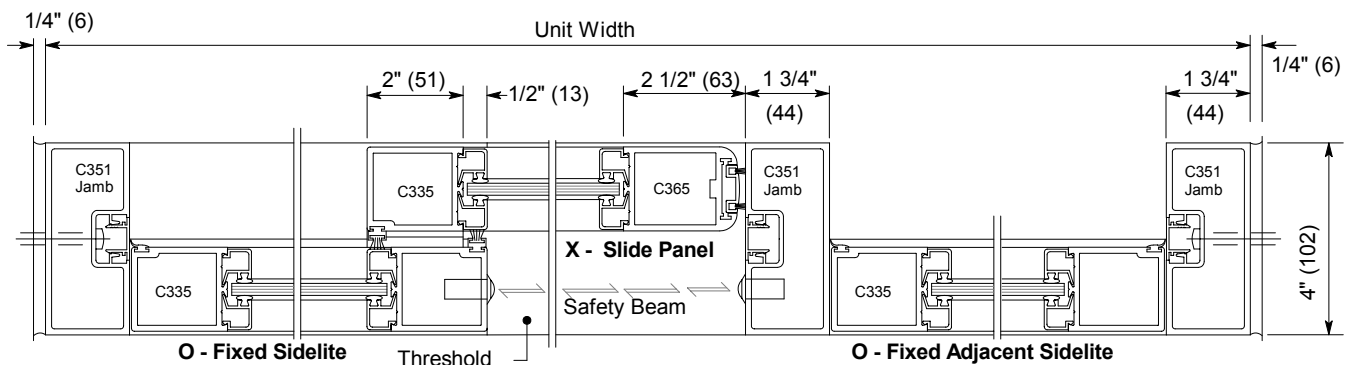
Horizontal Section
