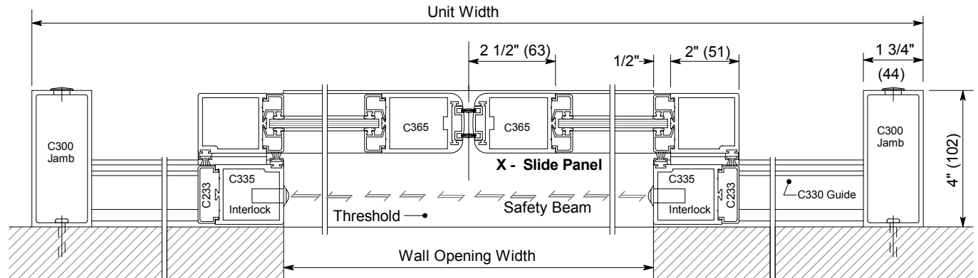
Horizontal Section
