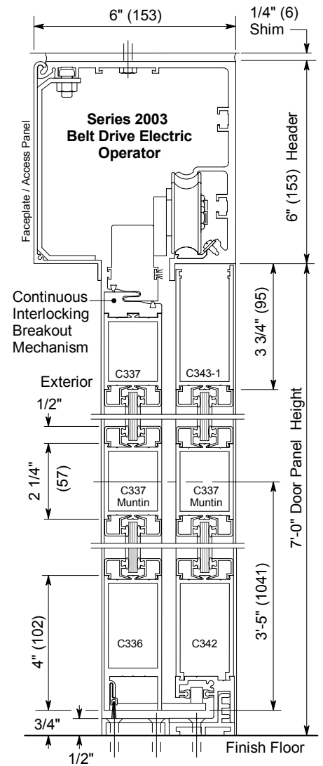
Vertical Section
