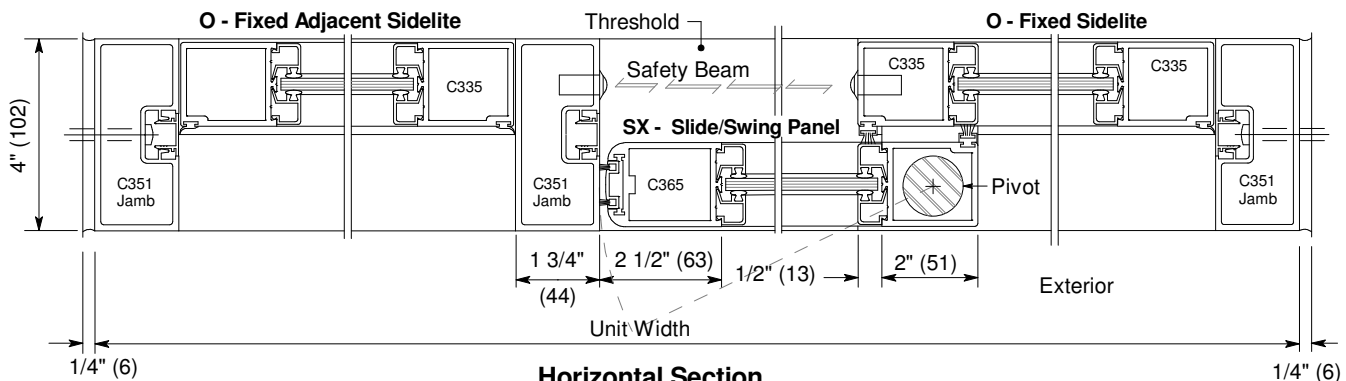
Horizontal Section
