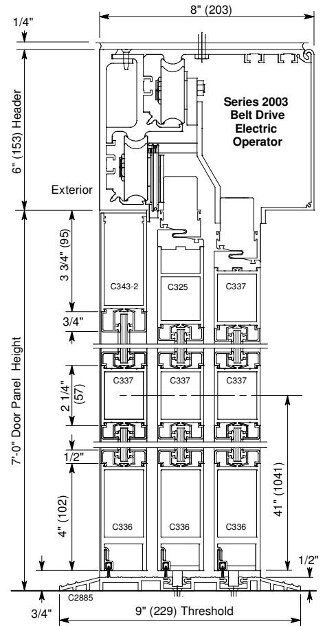
Vertical Section Door shown in open position
