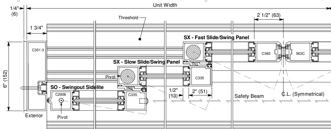
Exterior Elevation and Floor Plan
