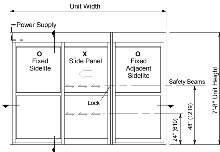
3 1/2" (89) Slide Opening Exterior Elevation and Floor Plan
