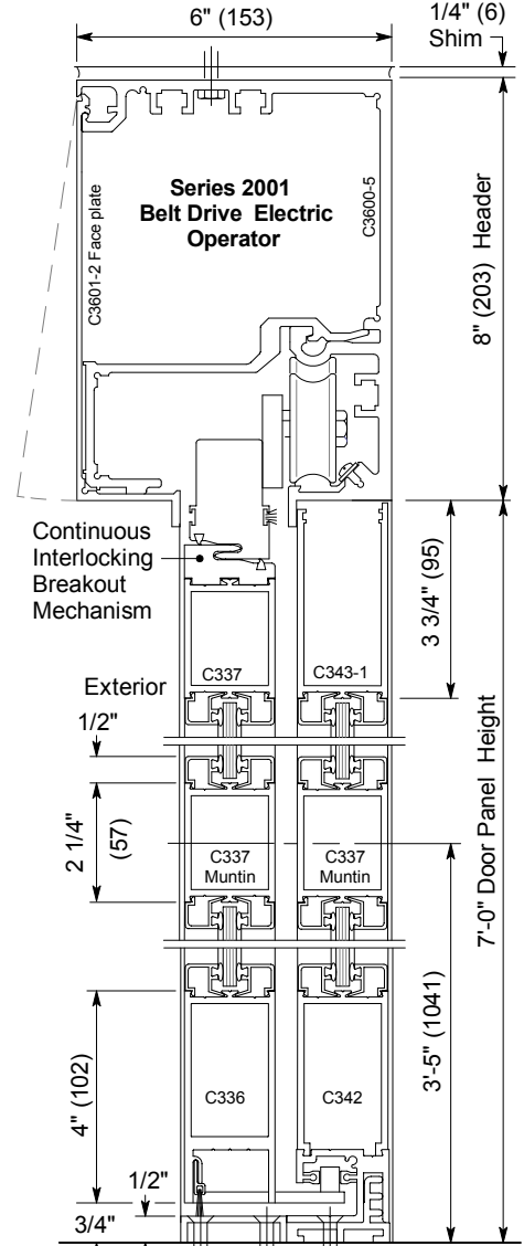
Vertical Section
