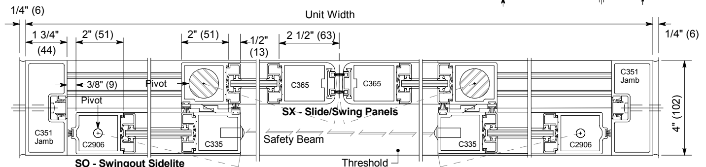
Horizontal Section
