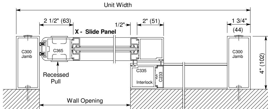
Horizontal Section Type X-P shown, P-X opposite
