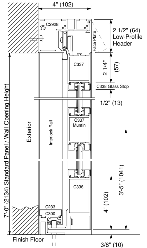
Vertical Section Door shown in open position
