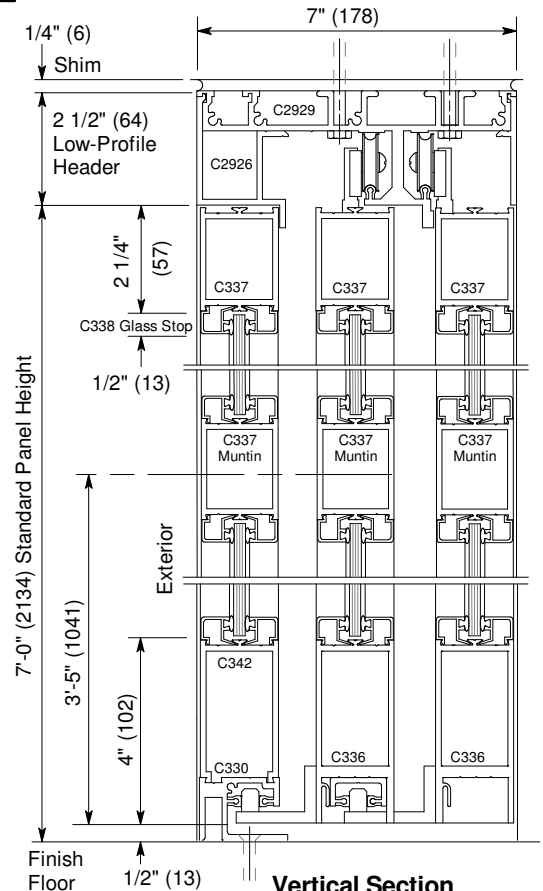
Vertical Section
