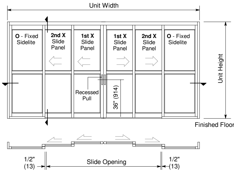
Exterior Elevation and Floor Plan
