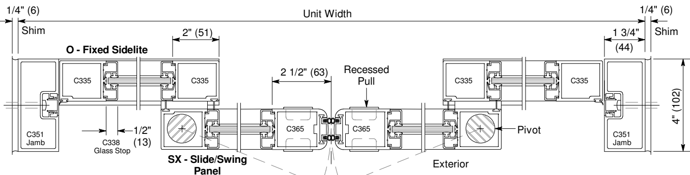
Horizontal Section
