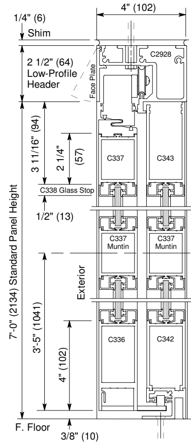
Vertical Section Door shown in open position
