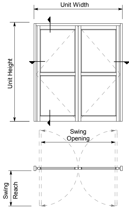
Exterior Elevation and Floor Plan
