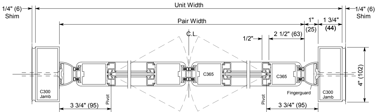
Horizontal Section
