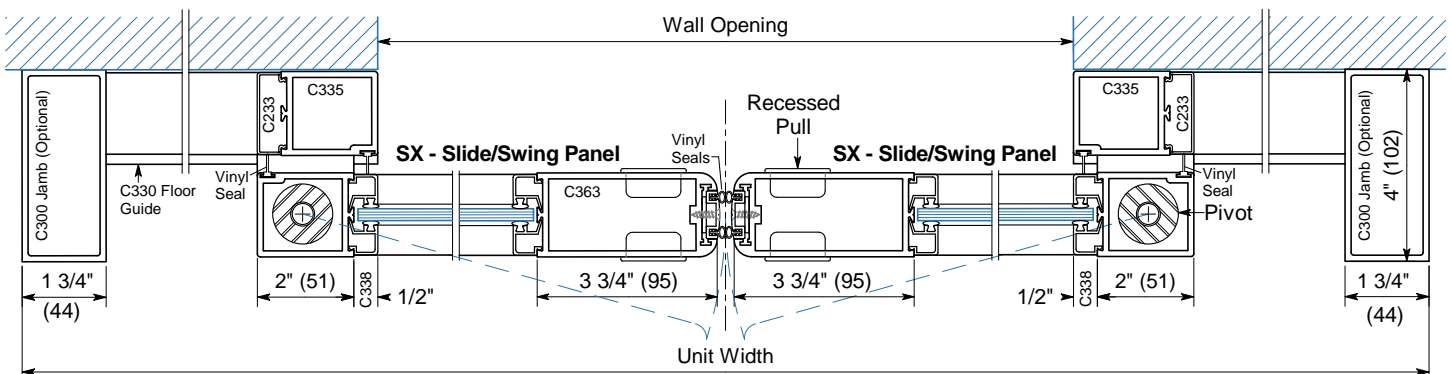
Horizontal Section
