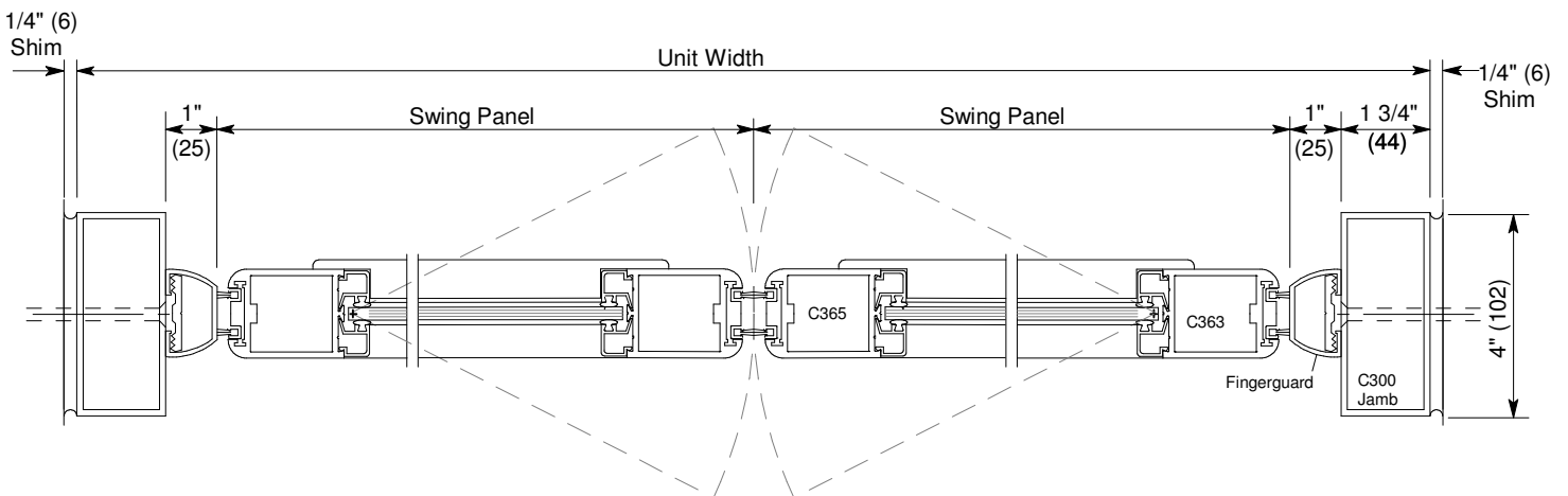
Horizontal Section
