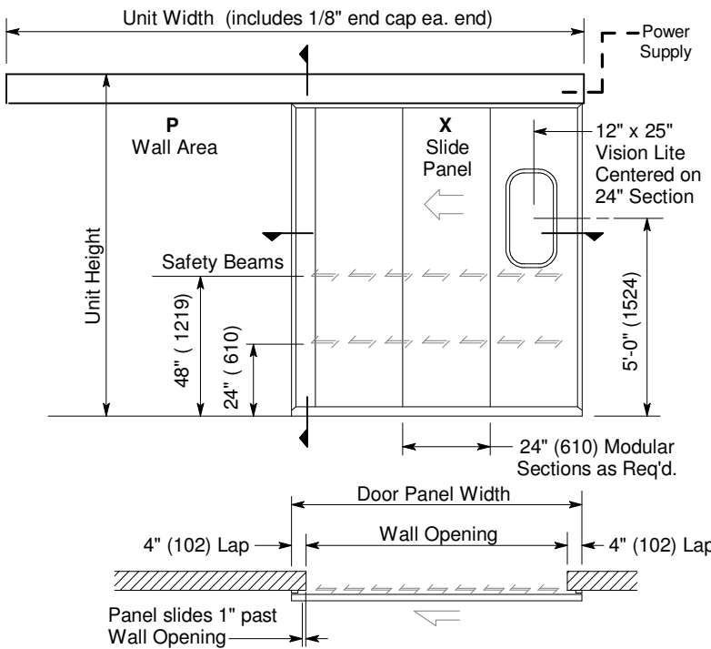
Exterior Elevation and Floor Plan
