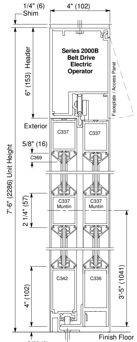
Vertical Section Door shown in open position
