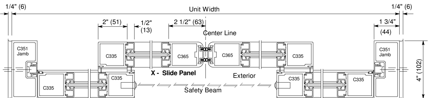
Horizontal Section
