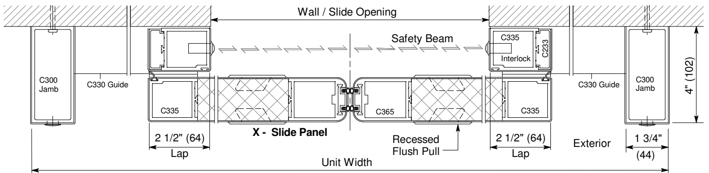
Horizontal Section
