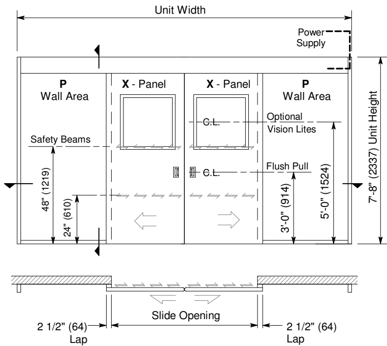
Exterior Elevation and Floor Plan
