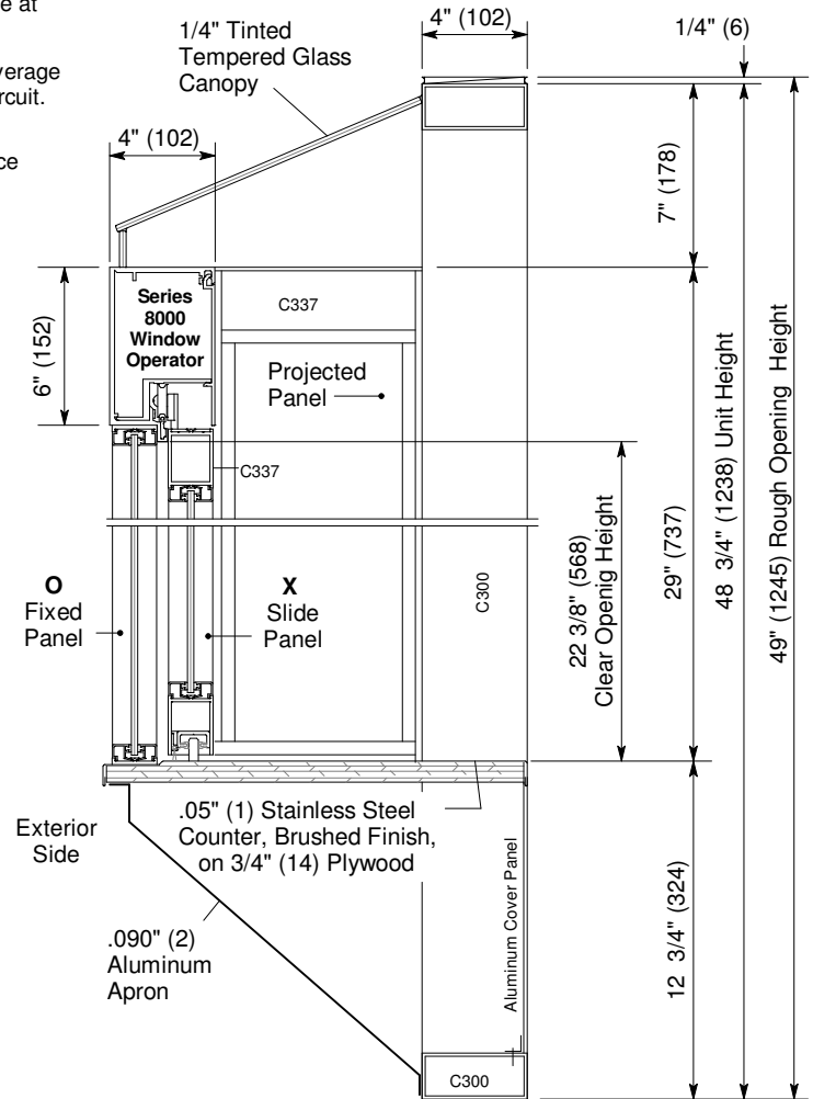
Vertical Section
