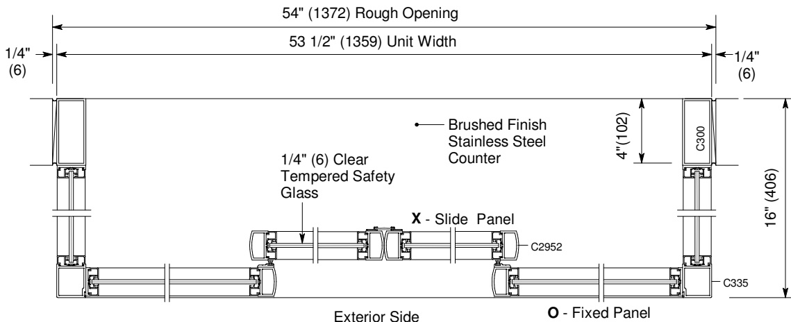
Horizontal Section
