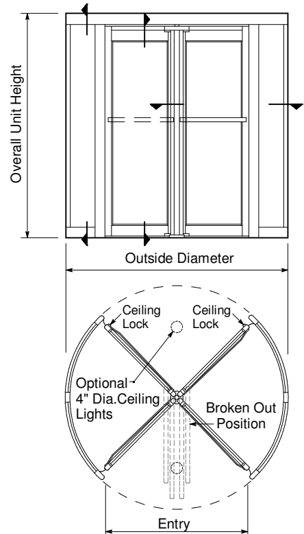
Floor Plan and Exterior Elevation
