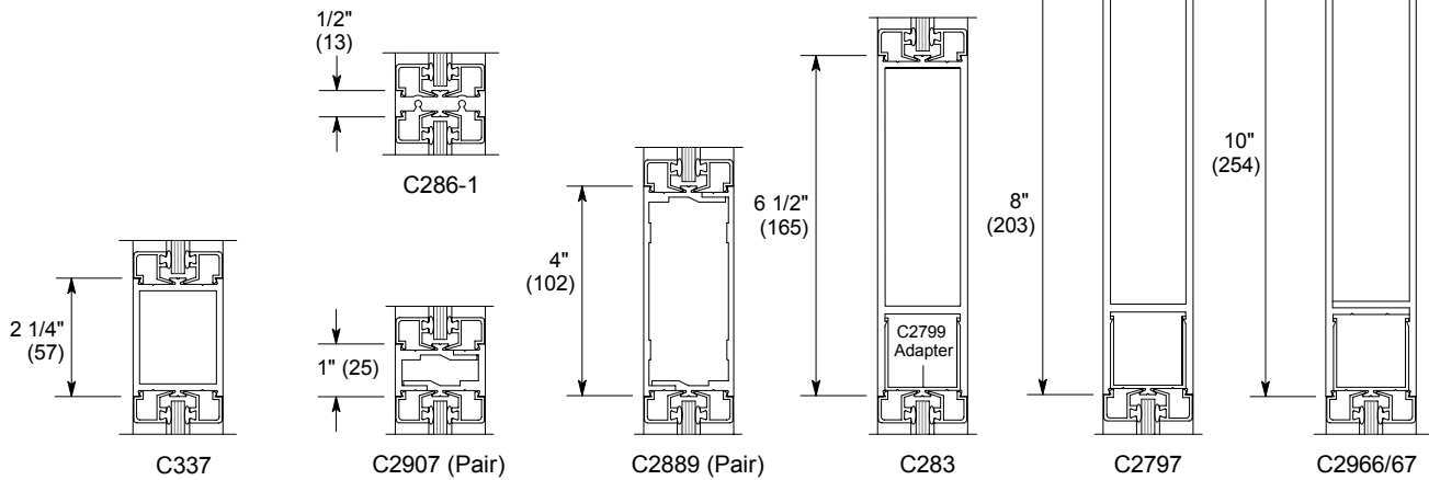
Optional Mid-Rails
