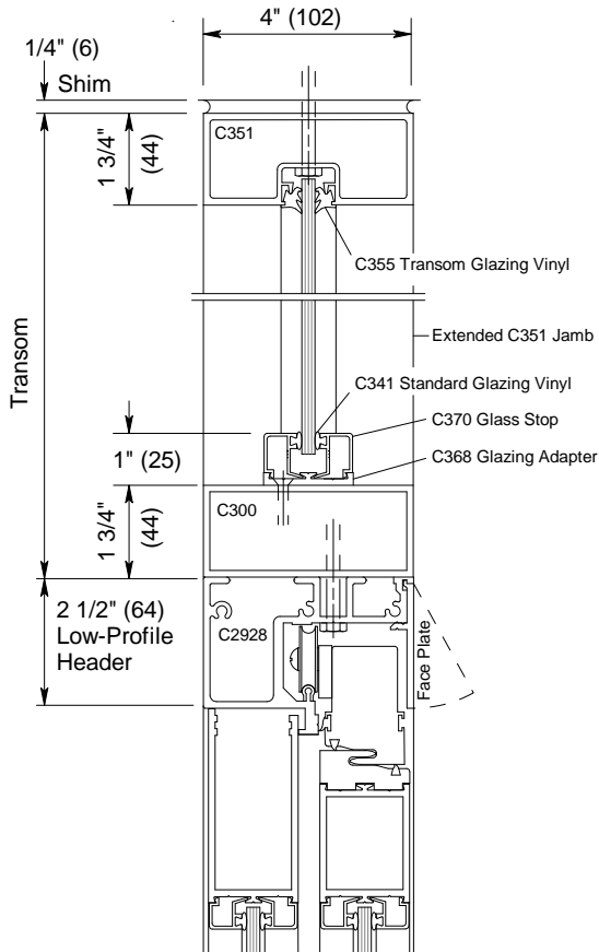
Low-Profile Header with Transom
