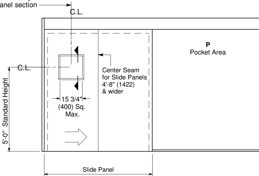
Units with Wide Panels
