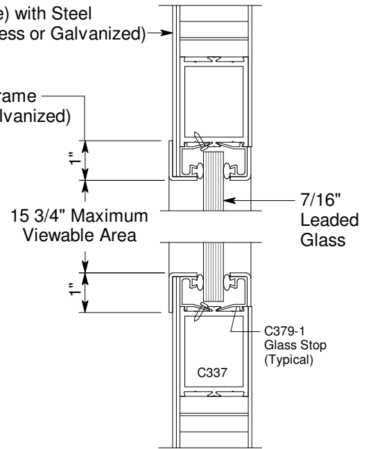
Typical Vertical Section
