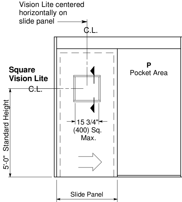
Units with Narrow Slide Panels
