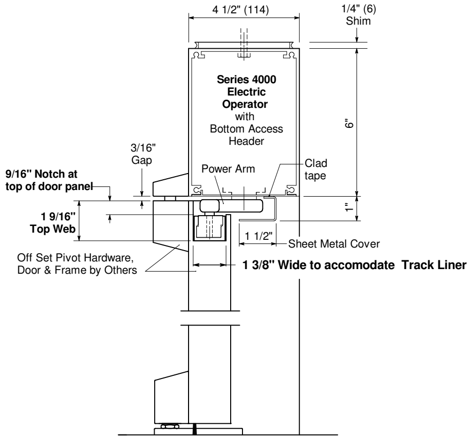
Vertical Section
