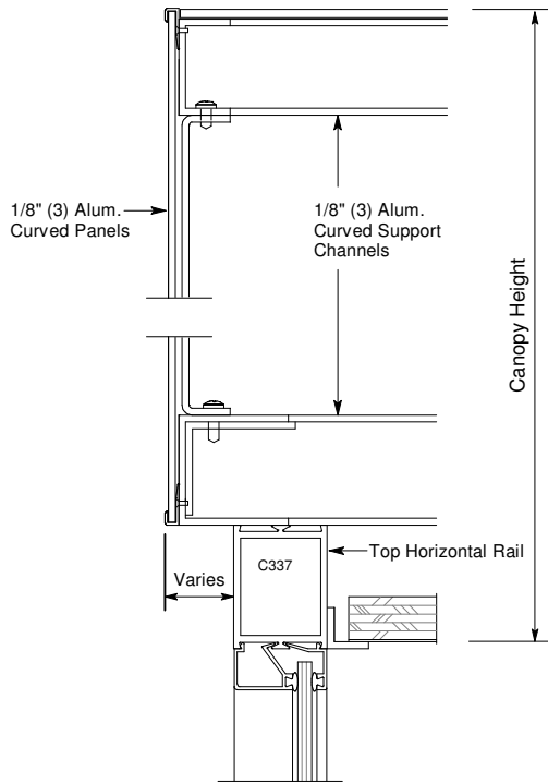
Section 'A' & 'A-1' at Top Horizontal Rail
