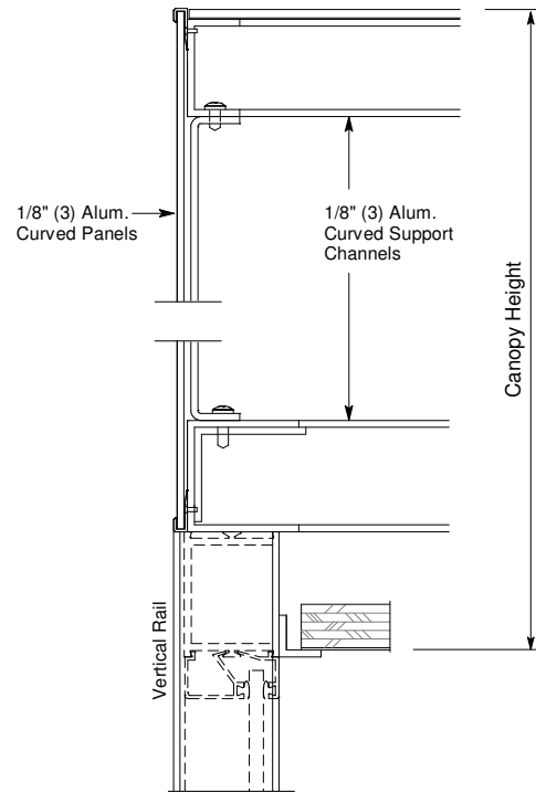
Section 'B' & 'B-1' at Vertical Rail
