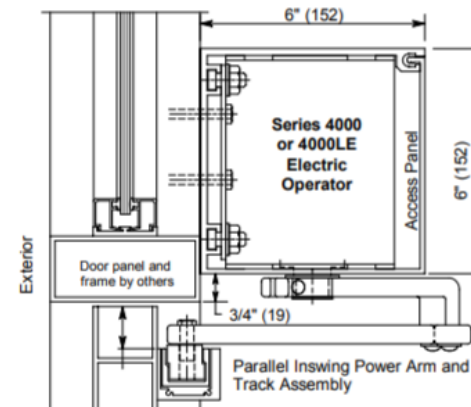
Parallel Inswing (power arm & slide track)
